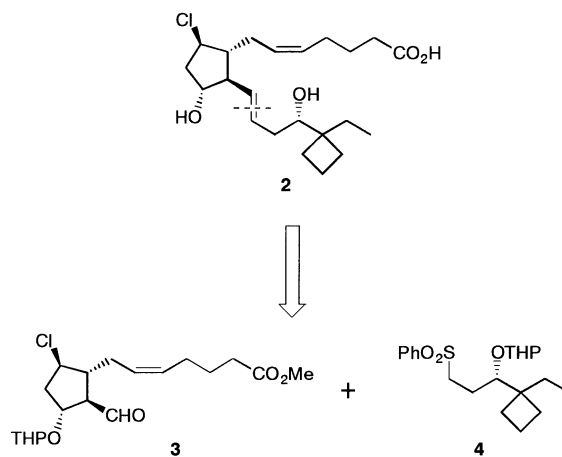
Scheme 1. Retrosynthesis of 2 .
