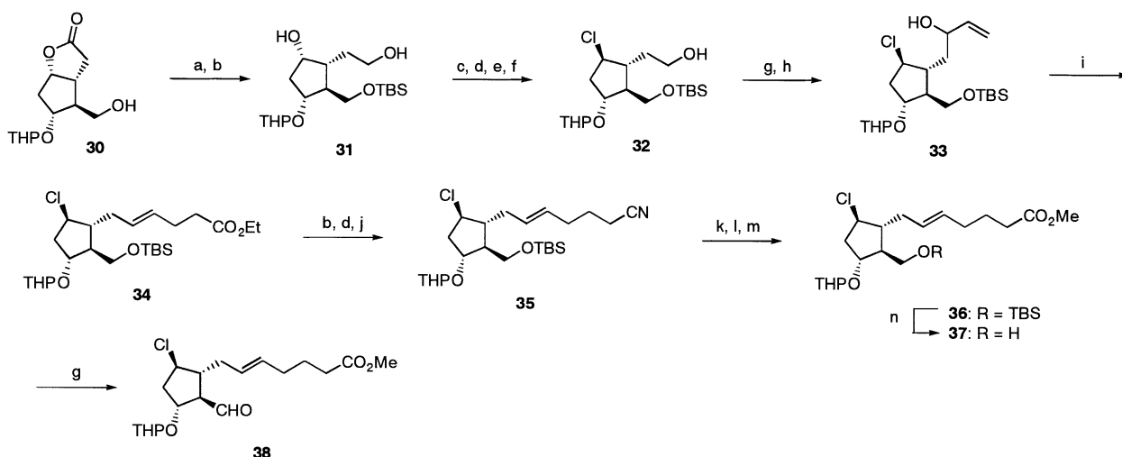
Scheme 4. Synthesis of 9 \beta -chloro 5( E )-aldehyde 38 . Reagents: (a) TBSCl, imidazole, DMF; (b) LiAlH 4 , THF; (c) Ac 2 O, collidine, CH 2 Cl 2 ; (d) TsCl, pyridine; (e) n -Bu 4 NCl, toluene; (f) NaOHaq, MeOH; (g) SO 3 -pyridine, Et 3 N, DMSO, CH 2 Cl 2 ; (h) CH 2 =CHMgBr, THF; (i) CH 3 CH(OEt) 3 , EtCO 2 H, 140 °C; (j) NaCN, DMSO, 100 °C; (k) i -Bu 2 AlH, CH 2 Cl 2 , then HClaq; (l) CrO 3 , H + , H 2 O; (m) CH 2 N 2 ; (n) n -Bu 4 NF, THF.
