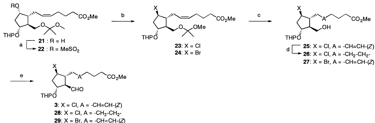
Scheme 3. Synthesis of 9 \beta -halo aldehyde 3 , 28 and 29 . Reagents: (a) MsCl, Et 3 N, CH 2 Cl 2 ; (b) n -Bu 4 NCl or n -Bu 4 NBr, Et 3 N, toluene, 60 °C; (c) HClaq, THF; (d) Pd/C, H 2 , MeOH; (e) SO 3 –pyridine, Et 3 N, DMSO.
