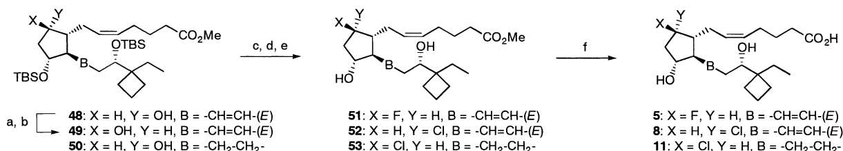
Scheme 6. Synthesis of other 9-halo PG analogues 5 , 8 and 11 . Reagents: (a) diethylazodicarboxylate, PPh 3 , HCOOH, THF; (b) NH 3 aq; (c) TsCl, pyridine; (d) n -Bu 4 NF or n -Bu 4 NCl, toluene; (e) HFAq, MeCN; (f) NaOHaq, MeOH.
