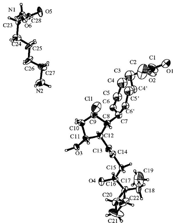
Fig 1. X-ray crystallographic structure of 2Ly .
