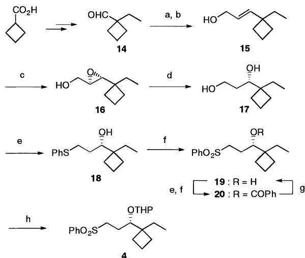
Scheme 2. Synthesis of an optically active \omega chain 4 . Reagents: (a) (EtO) 2 P(O)CH 2 CO 2 Et, NaH, THF; (b) i -Bu 2 AlH, THF, 0 °C; (c) t -BuOOH, Ti(OiPr) 4 , D-(–)-DIPT, CH 2 Cl 2 , –20 °C; (d) Na(MeOCH 2 CH 2 O) 2 AlH 2 , toluene; (e) TsCl, n -Bu 4 NBr, NaOHaq, toluene, then PhSH; (f) Oxone ® , MeOH, H 2 O; (g) PhCOCl, DMAP, pyridine; (h) Recrystallization from EtOH; (g) NaOHaq, MeOH; (h) DHP, p -TsOH, CH 2 Cl 2 .
