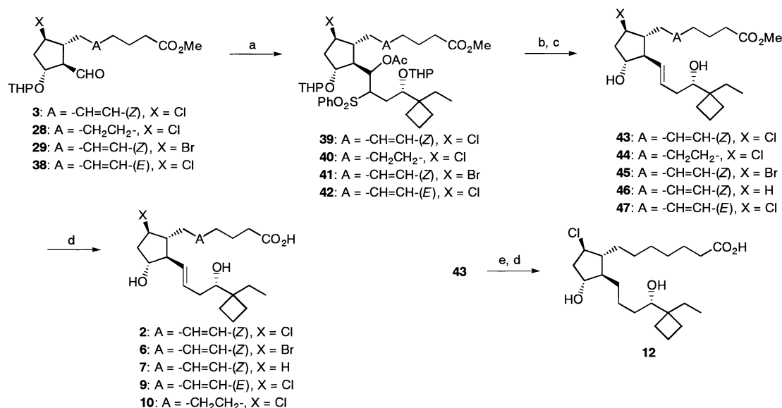
Scheme 5. Synthesis of 9 \beta -halo PG analogues 2 , 6 , 7 , 9 , 10 and 12 . Reagents: (a) 4 , n -BuLi, THF, -78 °C; (b) Mg (powdered, -50 mesh), TMSCl, MeOH; (c) p -TsOH, MeOH; (d) NaOHaq, MeOH; (e) Pd/C, H 2 , MeOH; (f) L-lysine, EtOH, EtOAc.
