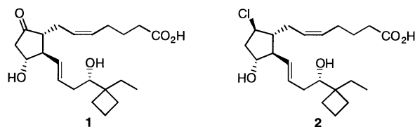
Chart 1. Structures of EP2-receptor agonists 1 and 2 .
